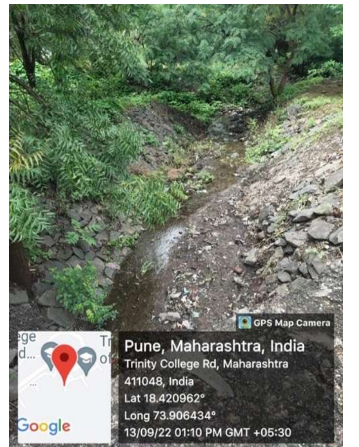
Channels to collect and transfer the rain/storm water
