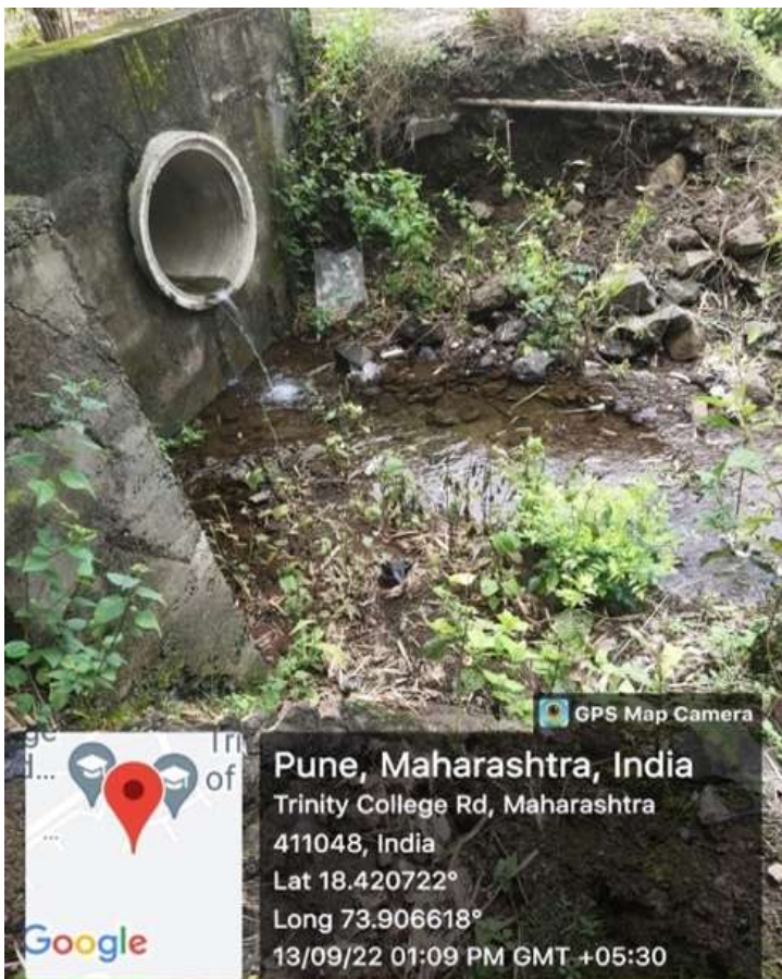
RCC pipe to collect and transfer the rain/storm water
